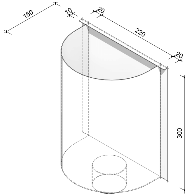
ISOMETRIC
